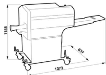
Dimensions Portio 140
